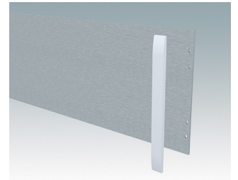
M5700023 Front panel trim 3U ABS (UL 94 HB) Light gray RAL 7035
