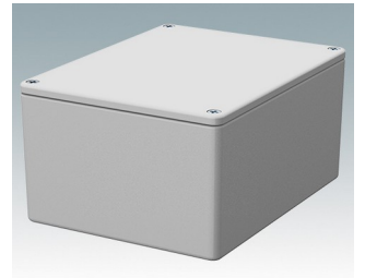
5007-17-WH Diecast Enclosure Diecast Aluminum Pure white RAL 9010 4.76"x3.74"x2.40" IP 65 opt.
