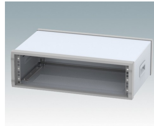
M6019305 INSTRUMET 19" 3Ux13.78" Aluminum Light gray/window gray RAL 7035/7040 6.18"x20.31"x13.78"
