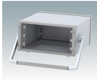
M6010315 INSTRUMET 10.5" 3Ux13.78" Aluminum Light gray/window gray RAL 7035/7040 6.18"x11.93"x13.78"
